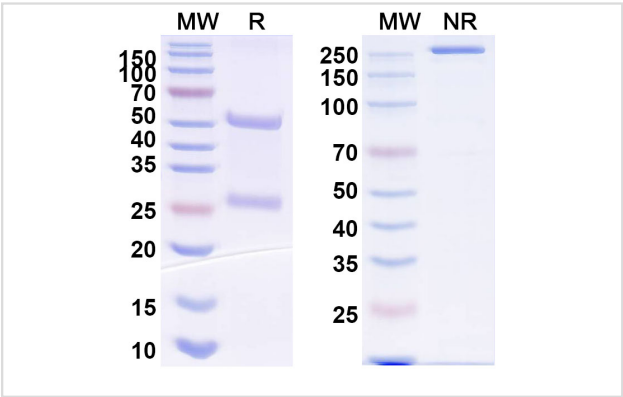
SDS-PAGE for Anti-Staphylococcus aureus Alpha-toxin/hly/AT Antibody
