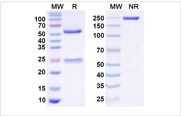
SDS-PAGE for Anti-Snake Venom Neutralizing Antibody
